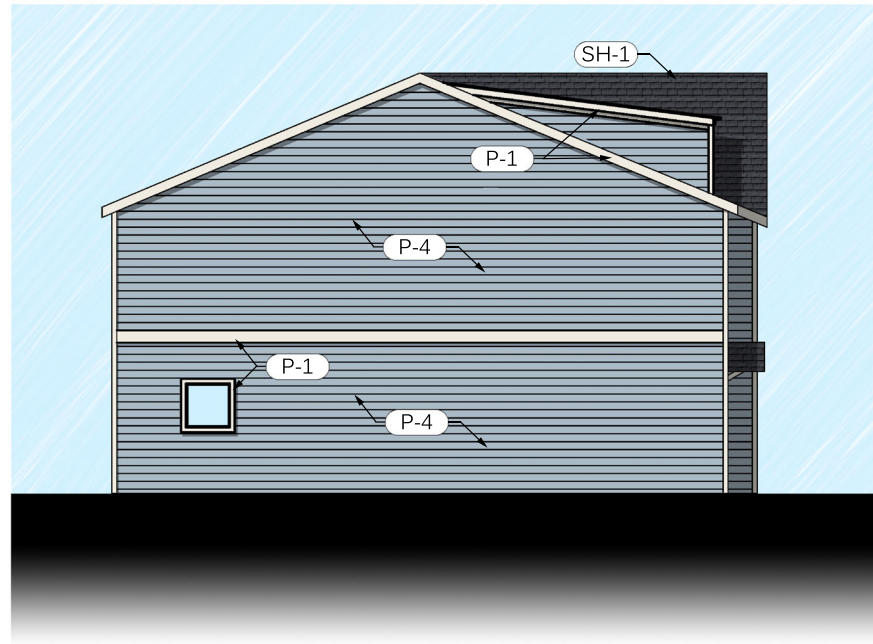
GARAGE ENTRY LEFT SIDE ELEVATION
